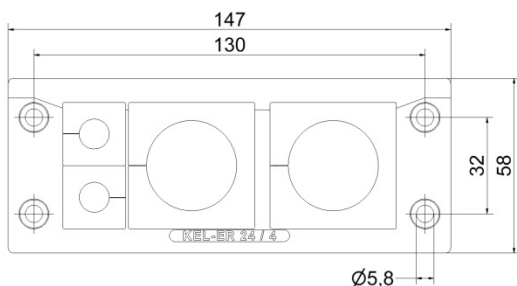
KEL-ER 24/4 Art.No.SFKD-R003
