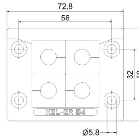
KEL-ER B4 Art.No.SFKD-R005
