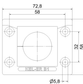
KEL-ER B Art.No.SFKD-R004
