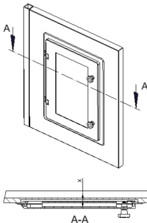
Framed window SF034
