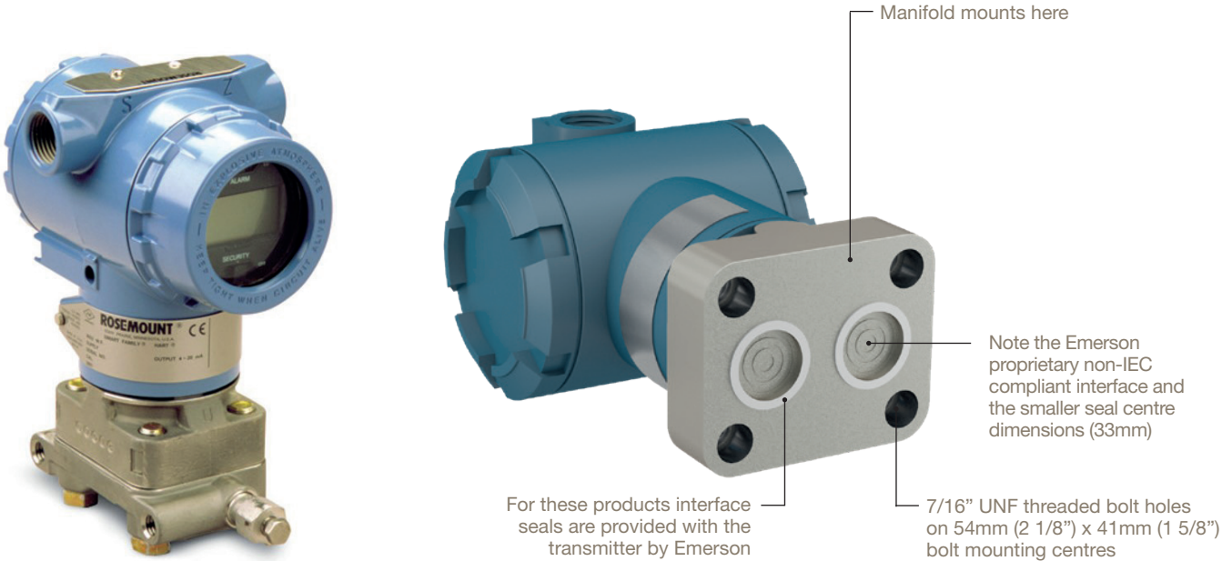
3051 DP transmitter, shown with the Emerson flange adapter in lieu of a manifold. A directly mounted Parker Coplanar™ manifold, replaces this.
